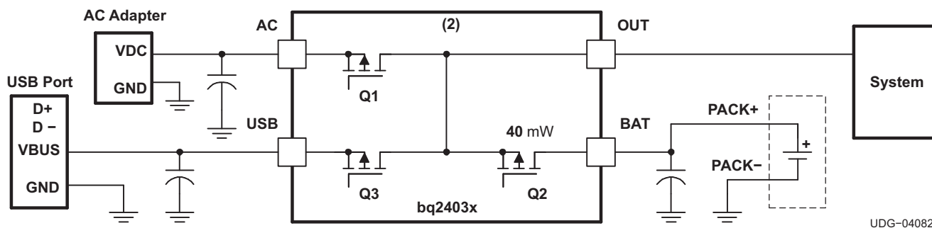
Figure 3. Power-Path Management
