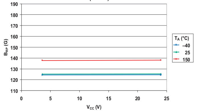
Release Point versus Supply Voltage (A3242)
