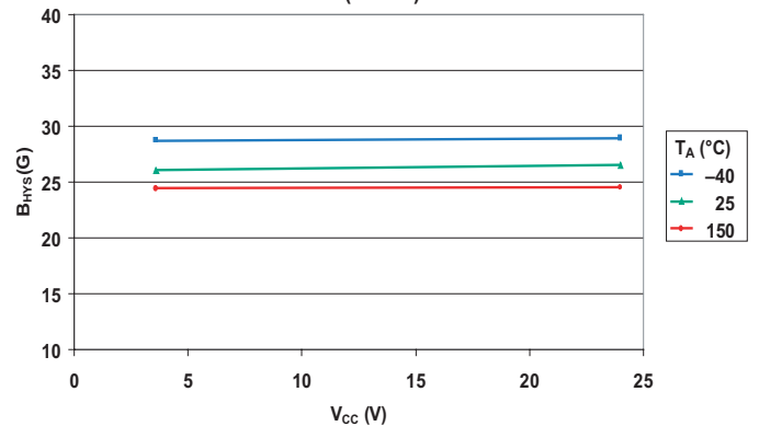
Hysteresis versus Supply Voltage (A3242)
