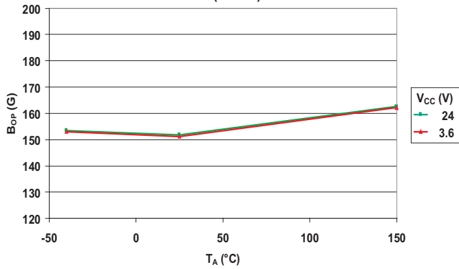
Operate Point versus Ambient Temperature (A3242)
