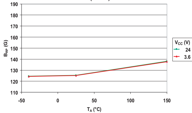
Release Point versus Ambient Temperature (A3242)
