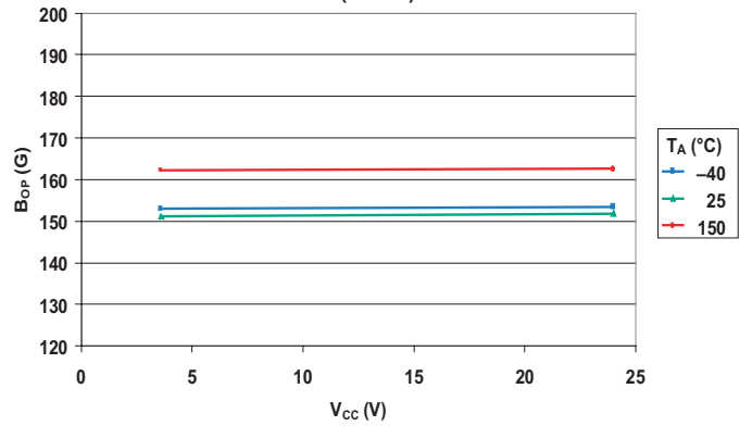
Operate Point versus Supply Voltage (A3242)
