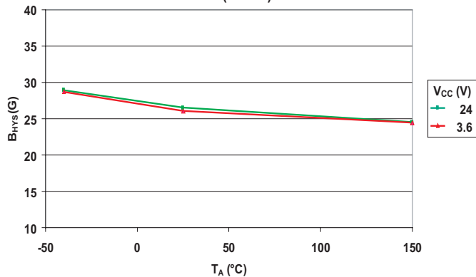
Hysteresis versus Ambient Temperature (A3242)
