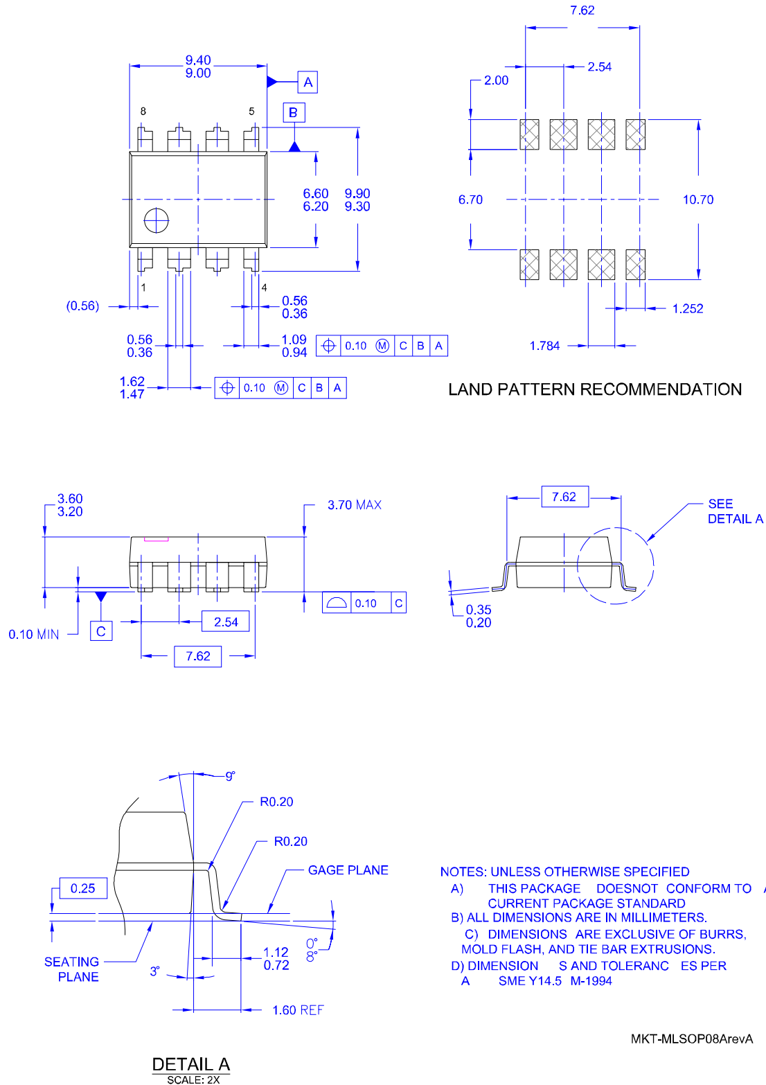
Figure 25. 8-Lead LSOP
