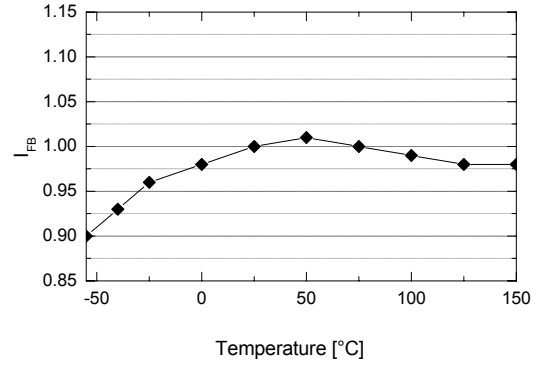
Figure 11. Feedback Source Current ( I_{\text{FB}} ) vs. T_A
