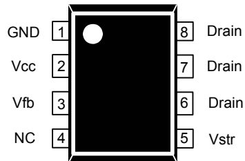
Figure 3. Pin Configuration (Top View)
