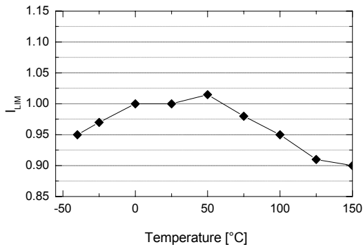
Figure 10. Peak Current Limit ( I_{\text{LIM}} ) vs. T_A
