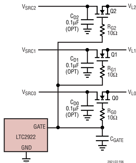
Figure 6. Ramping and Damping Components on GATE Pin
