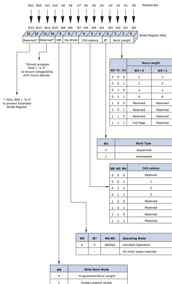
Figure 4: Mode Register Definition
