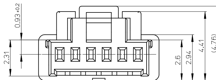
VIEW "D"
