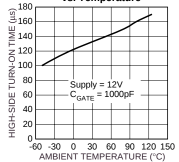
High-Side Turn-On Time vs. Temperature
