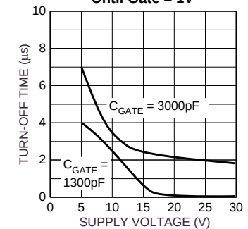
High-Side Turn-Off Time Until Gate = 1V
