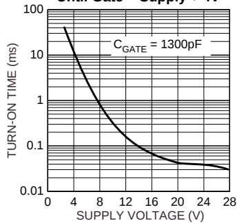
High-Side Turn-On Time Until Gate = Supply + 4V
