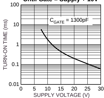
High-Side Turn-On Time Until Gate = Supply + 10V
