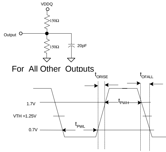
2.5V LVTTTL OUTPUT WAVEFORM
