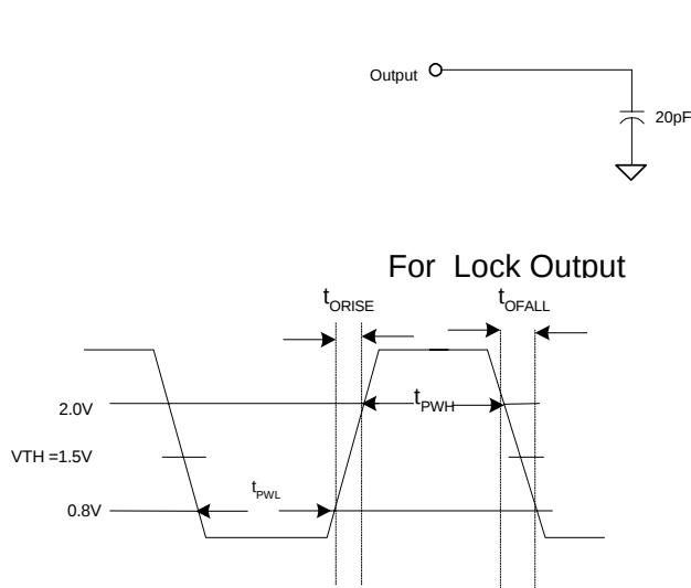
3.3V LVTTTL OUTPUT WAVEFORM
