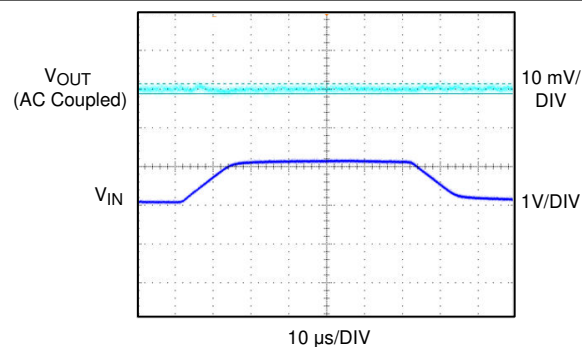
Figure 5-8. Line Regulation
