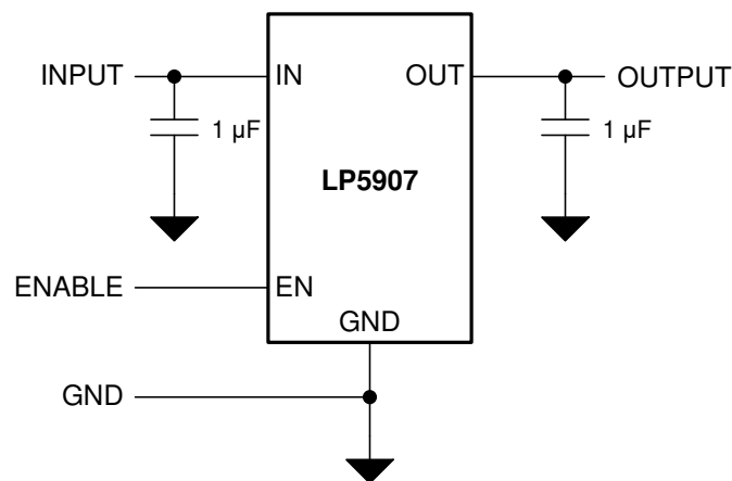
Simplified Schematic
