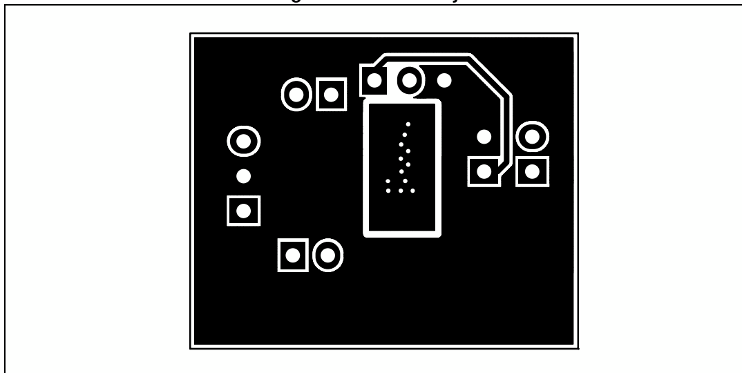
Figure 69. Top layer
