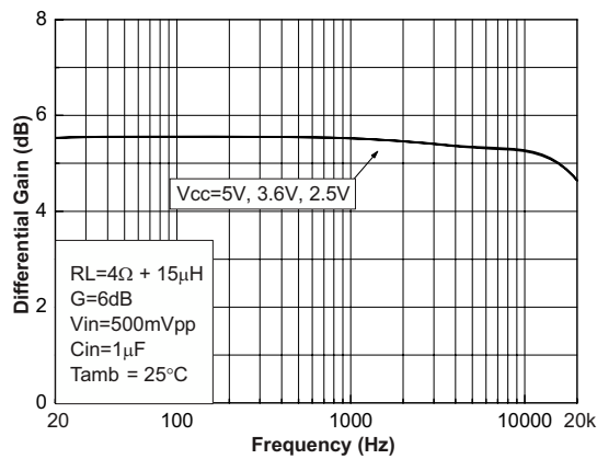
Figure 50. Gain vs. frequency
