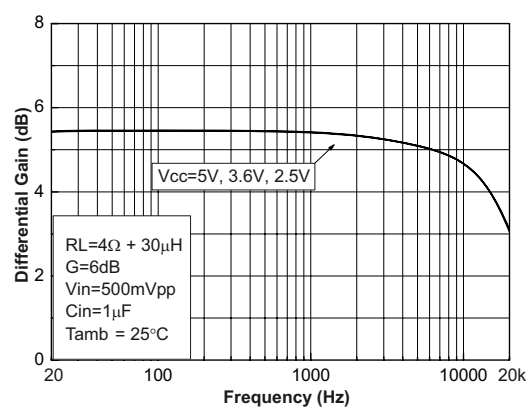
Figure 51. Gain vs. frequency
