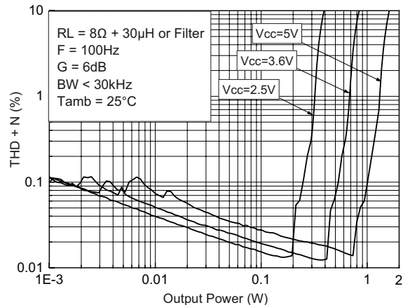
Figure 33. THD+N vs. output power
