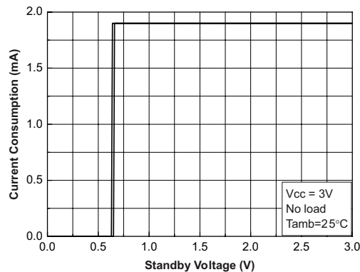
Figure 6. Current consumption vs. standby voltage
