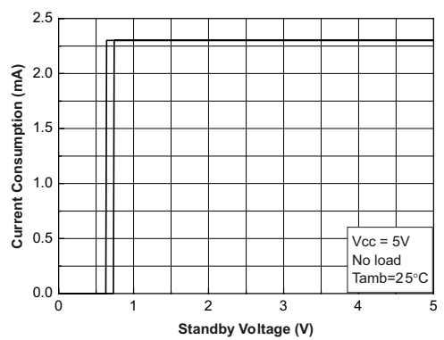
Figure 5. Current consumption vs. standby voltage
