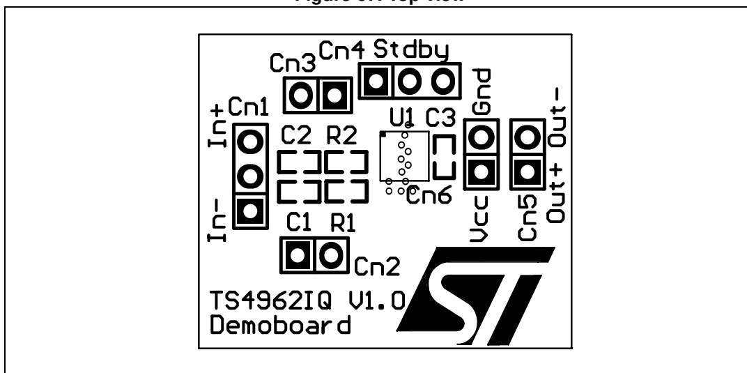
Figure 67. Top view
