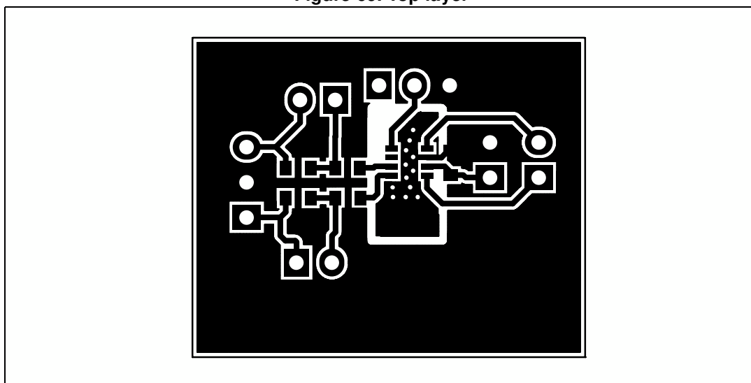
Figure 69. Top layer
