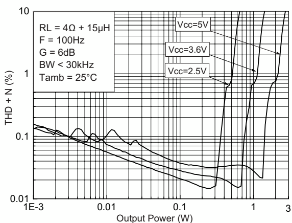
Figure 28. THD+N vs. output power
