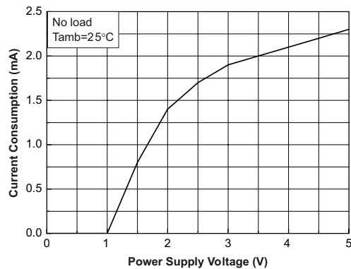
Figure 4. Current consumption vs. power supply voltage
