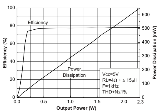
Figure 8. Efficiency vs. output power
