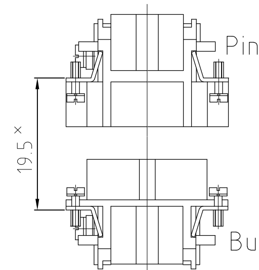
× distance for a safe contact max: max: 21 mm
