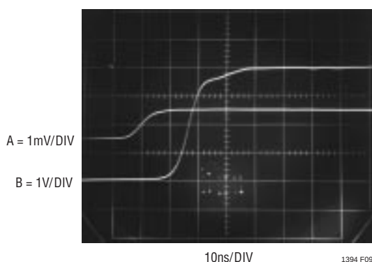
Figure 9. Parallel Path Comparator Shows 18ns Response (Trace B) to 500\mu\text{V} Overdrive (Trace A)
