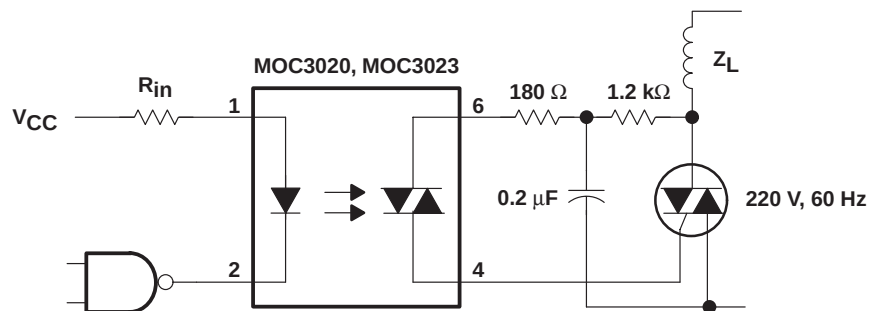
Figure 6. Inductive Load With Sensitive-Gate Triac
