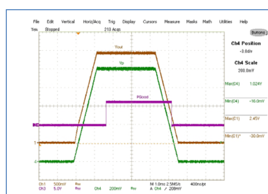
Figure 44: Voltage tracking using Vp pin Ch1:V out , Ch3:PGood, Ch4:V p
