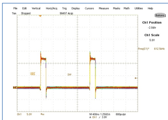
Figure 34: Inductor node at 16A load, Ch1:SW node
