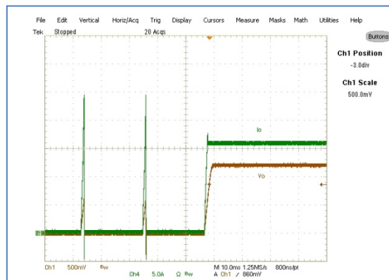
Figure 35: Short Circuit Recovery, Ch1:Vout, Ch4:Iout (5A/Div)
