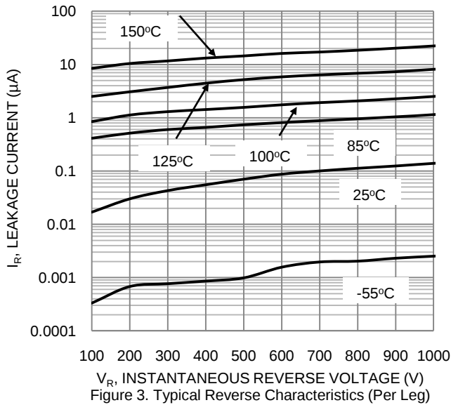
Figure 3. Typical Reverse Characteristics (Per Leg)
