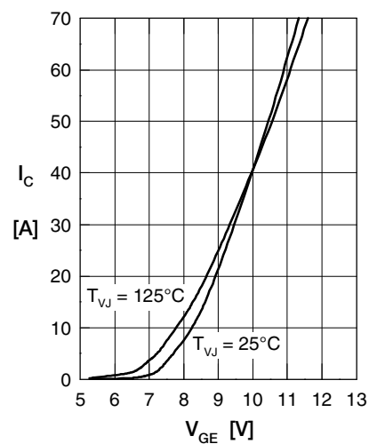
Fig. 3 Typ. tranfer characteristics
