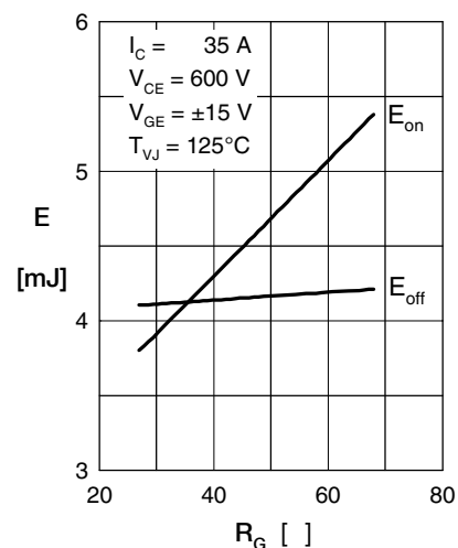
Fig. 6 Typ. switching energy versus gate resistance
