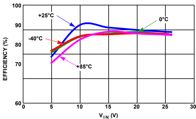
FIGURE 6. EFFICIENCY vs V_{IN} vs TEMPERATURE AT 20mA
