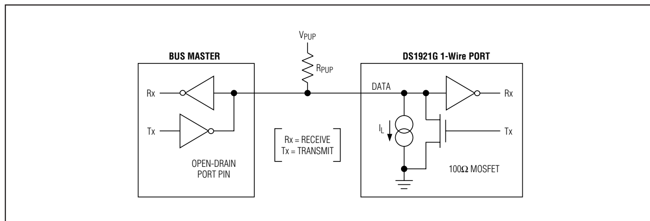
Figure 12. Hardware Configuration
