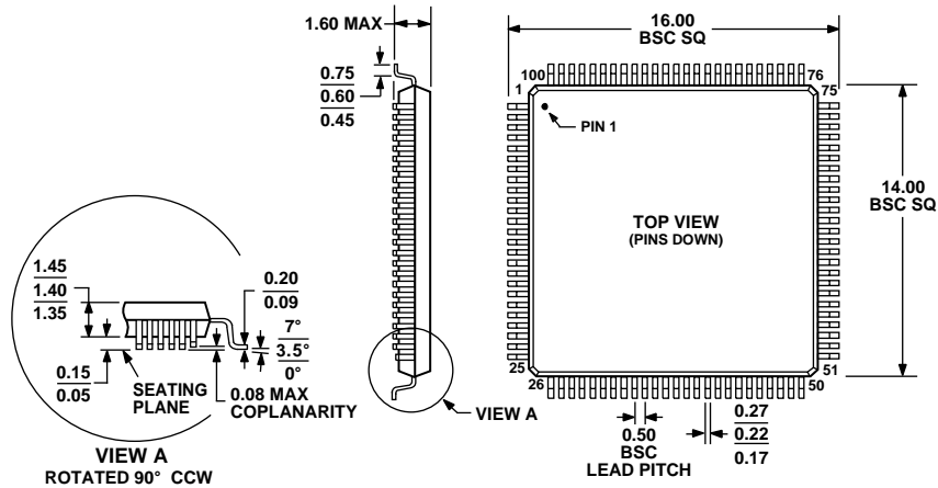
Figure 60. 100-Lead Low Profile Quad Flat Package [LQFP] (ST-100) Dimension shown in millimeters
