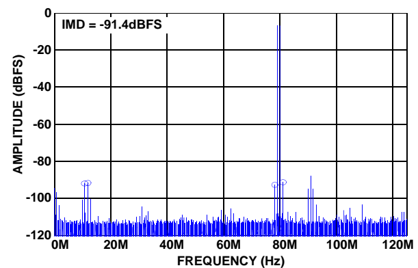
FIGURE 20. TWO-TONE SPECTRUM @ 170MHz
