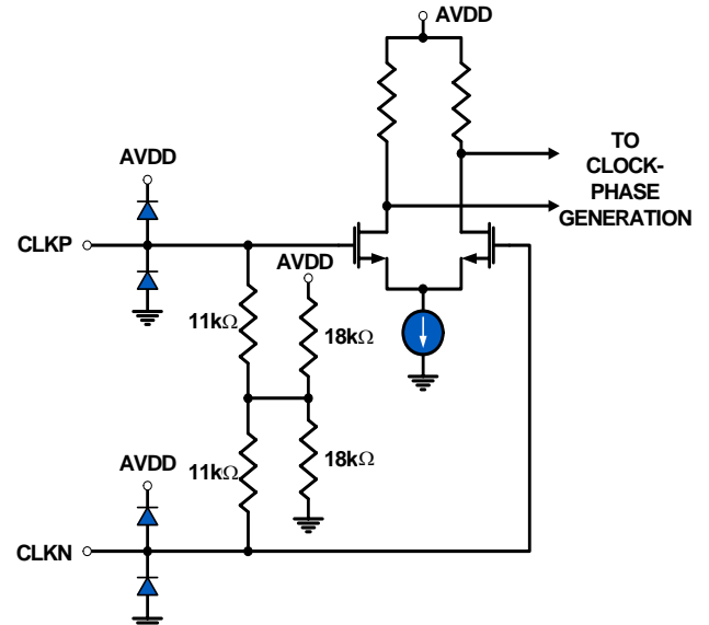
FIGURE 42. CLOCK INPUTS
