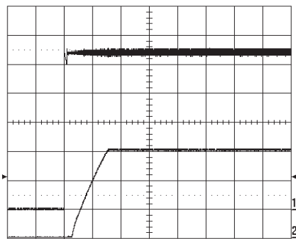
Start-up at I_o=3.33 A resistive load at T_{Pcb}=+25 °C, V_{in}=27 V. Start enabled by connecting V_{in} . Top trace: input voltage (5 V/div.). Bottom trace: output voltage (5 V/div.). Time scale: 5 ms/div.
