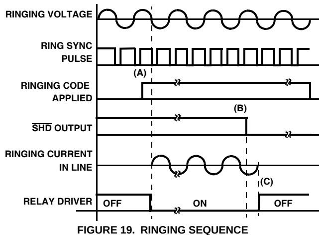
FIGURE 19. RINGING SEQUENCE
