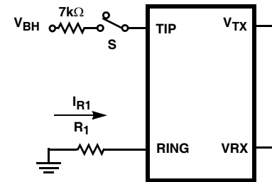
FIGURE 11. TIPX VOLTAGE
