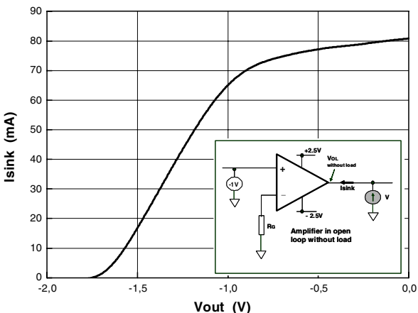
Figure 40. I_{sink}
