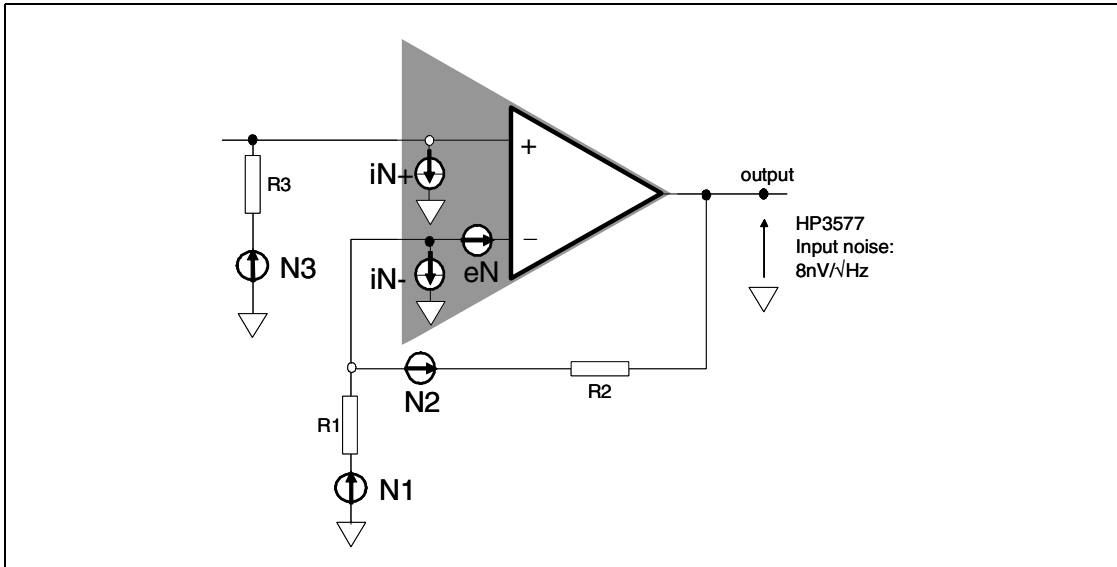
Figure 45. Noise model
