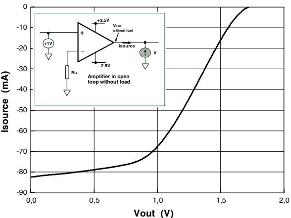
Figure 42. I_{source}
