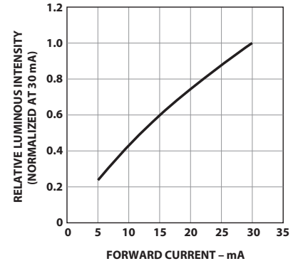
Figure 4. Relative intensity vs. forward current (InGaP)
