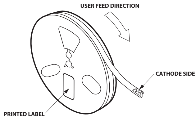
Figure 14. Reeling orientation
