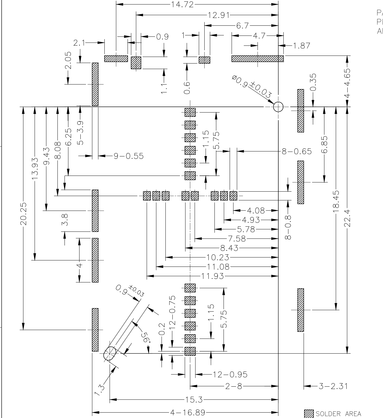
REFERENCE PCB LAYOUT (TOLERANCE : +/-0.05) FROM MOUNTING SURFACE
