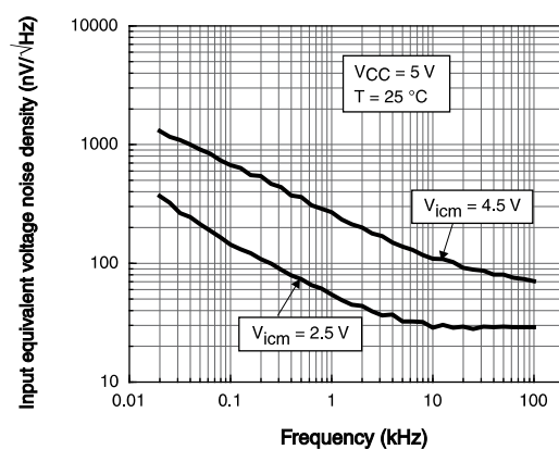
Figure 18: Noise vs. frequency at V_{CC} = 5\text{ V}
