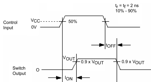
FIGURE 1. Turn ON/OFF Timing
