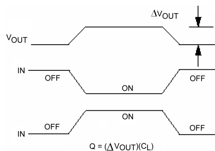
FIGURE 2. Charge Injection
