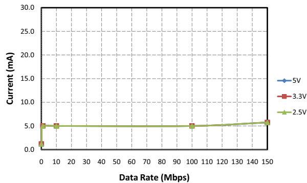
Figure 9. Si8660 Typical V_{DD1} Supply Current vs. Data Rate 5, 3.3, and 2.5 V Operation
