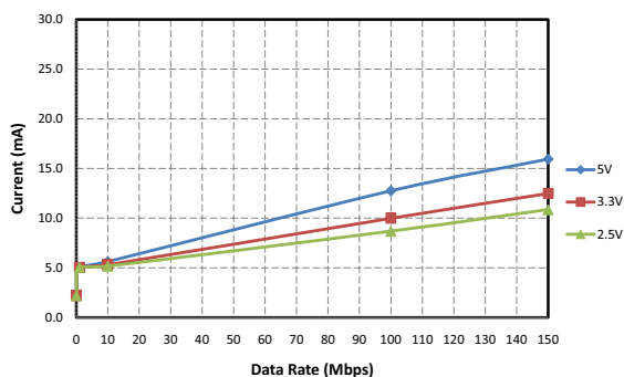
Figure 11. Si8662 Typical V_{DD1} Supply Current vs. Data Rate 5, 3.3, and 2.5 V Operation (15 pF Load)
