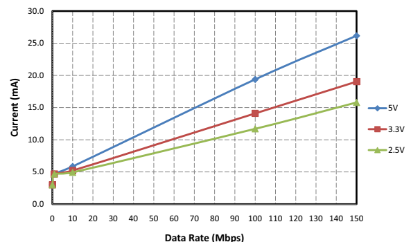
Figure 14. Si8662 Typical V_{DD2} Supply Current vs. Data Rate 5, 3.3, and 2.5 V Operation (15 pF Load)
