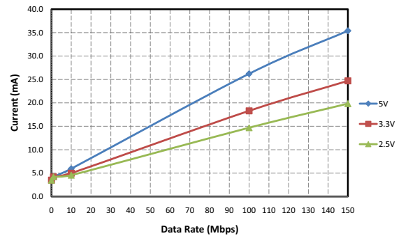
Figure 12. Si8660 Typical V_{DD2} Supply Current vs. Data Rate 5, 3.3, and 2.5 V Operation (15 pF Load)
