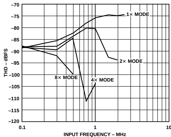
Figure 15. THD vs. Input Frequency ( f_{\text{CLOCK}} = 10 MSPS)
