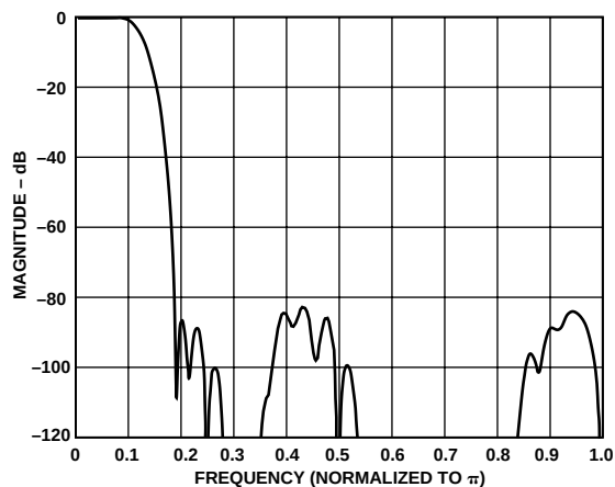
Figure 1a. 8× FIR Filter Frequency Response
