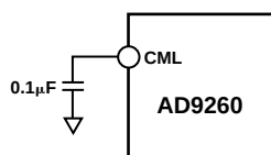
Figure 59. CML Decoupling
