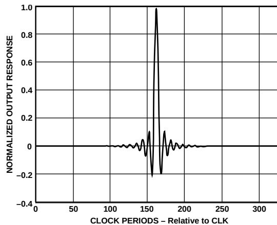
Figure 1b. 8× FIR Filter Impulse Response
