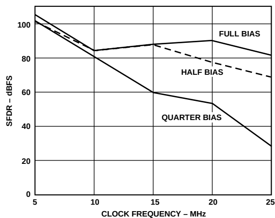
Figure 42. SFDR vs. Clock Rate ( f_{IN} = 500 kHz in 4 \times Mode)
