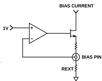
Figure 63. Simplified Bias Pin Circuitry
