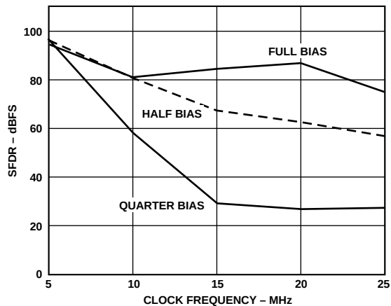
Figure 43. SFDR vs. Clock Rate ( f_{IN} = 1.0 MHz in 2 \times Mode)
