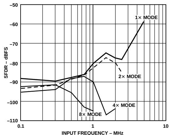
Figure 13. SFDR vs. Input Frequency ( f_{\text{CLOCK}} = 20 MSPS)
