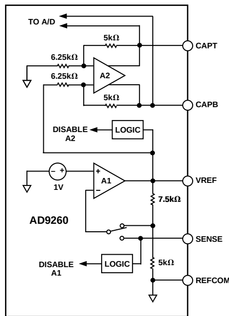
Figure 60. Simplified Reference
