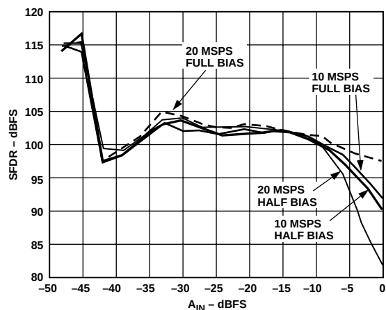
Figure 47. Single-Tone SFDR vs. Amplitude ( f_{IN} = 100 kHz, 8x Mode)
