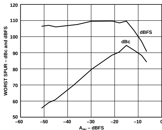
Figure 52. Two-Tone SFDR ( F_1 = 1.9 MHz, F_2 = 2.1 MHz, 4x Mode 20 MSPS)
