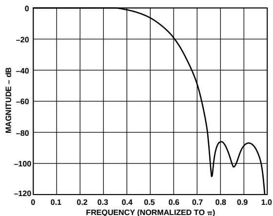
Figure 3a. 2× FIR Filter Frequency Response
