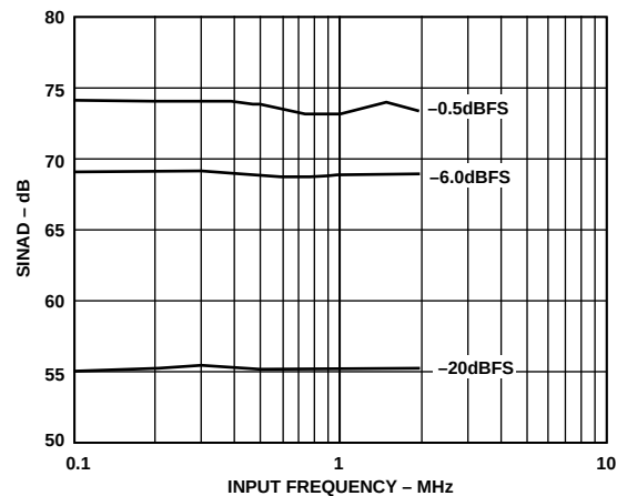
Figure 32. SINAD vs. Input Frequency ( f_{\text{CLOCK}} = 10 \text{ MSPS} )
