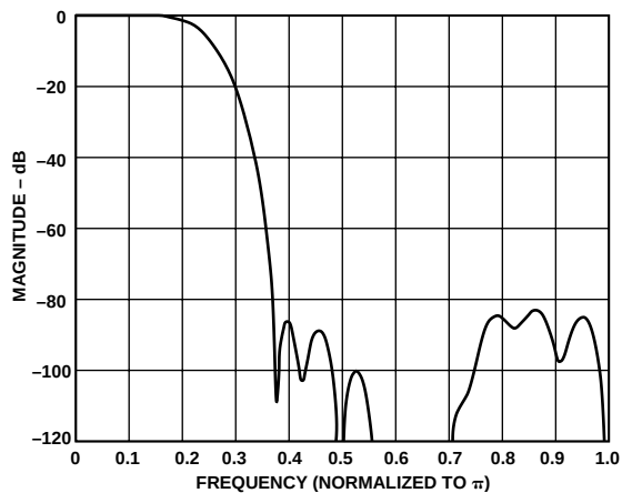
Figure 2a. 4× FIR Filter Frequency Response
