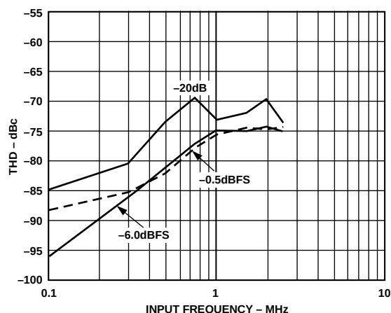
Figure 39. THD vs. Input Frequency ( f_{\text{CLOCK}} = 10 \text{ MSPS} )
