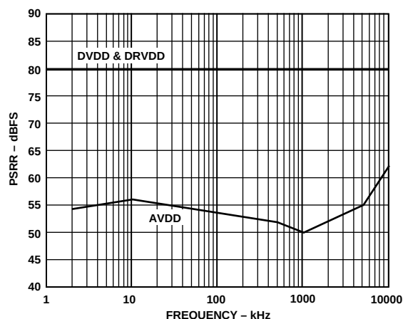
Figure 66. AD9260 PSRR vs. Frequency (8 × Mode)
