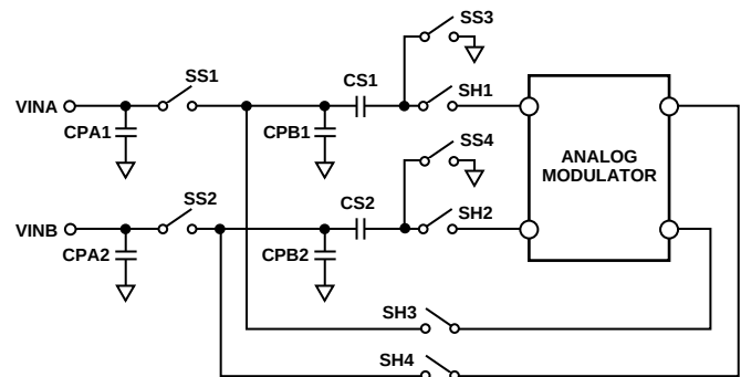
Figure 55. Detailed Analog Input Structure
