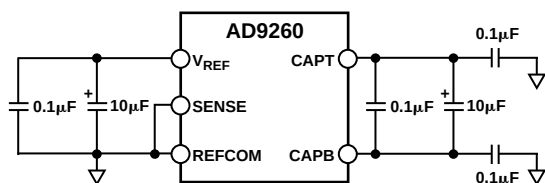
Figure 61. Recommended Reference Decoupling Network
