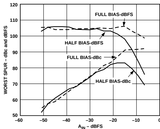
Figure 51. Two-Tone SFDR ( F_1 = 0.95 kHz, F_2 = 1.05 MHz, 8x Mode 20 MSPS)
