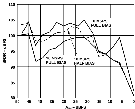
Figure 48. Single-Tone SFDR vs. Amplitude ( f_{IN} = 1.0 MHz, 2x Mode)
