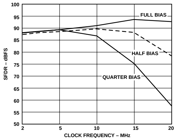
Figure 41. SFDR vs. Clock Rate ( f_{IN} = 100 kHz in 8 \times Mode)
