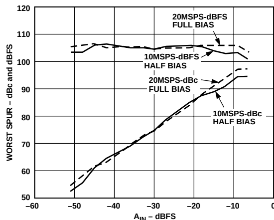
Figure 50. Two-Tone SFDR ( F_1 = 475 kHz, F_2 = 525 MHz, 8x Mode)
