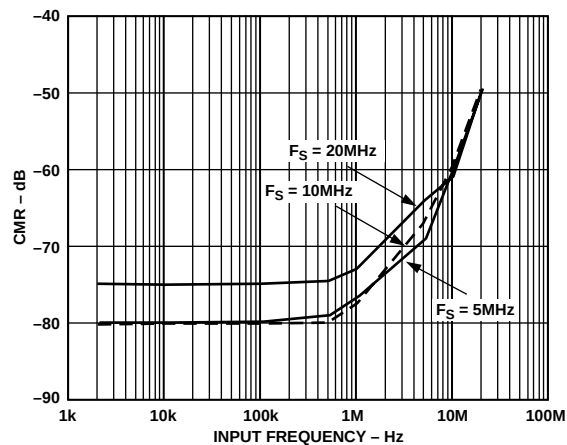
Figure 45. CMR vs. Input Frequency ( V_{CML} = 2 V p-p, 1 \times Mode)
