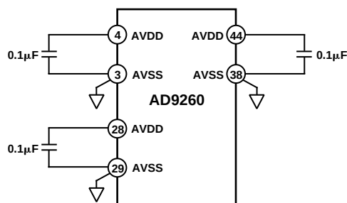
Figure 67. Analog Supply Decoupling
