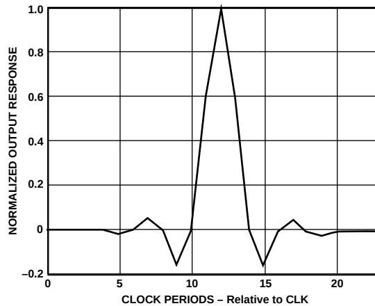
Figure 3b. 2× FIR Filter Impulse Response
