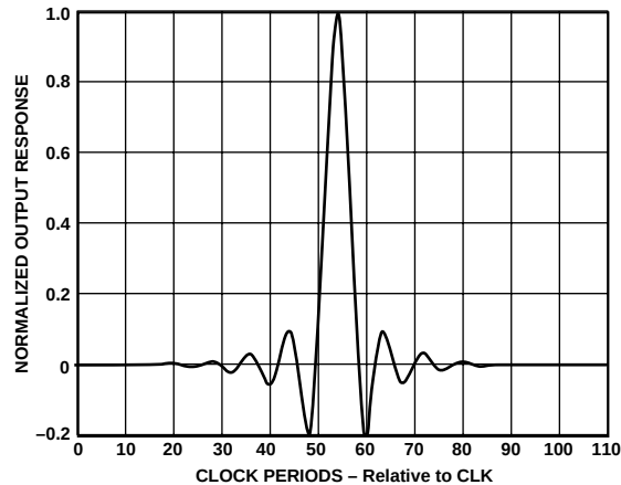
Figure 2b. 4× FIR Filter Impulse Response
