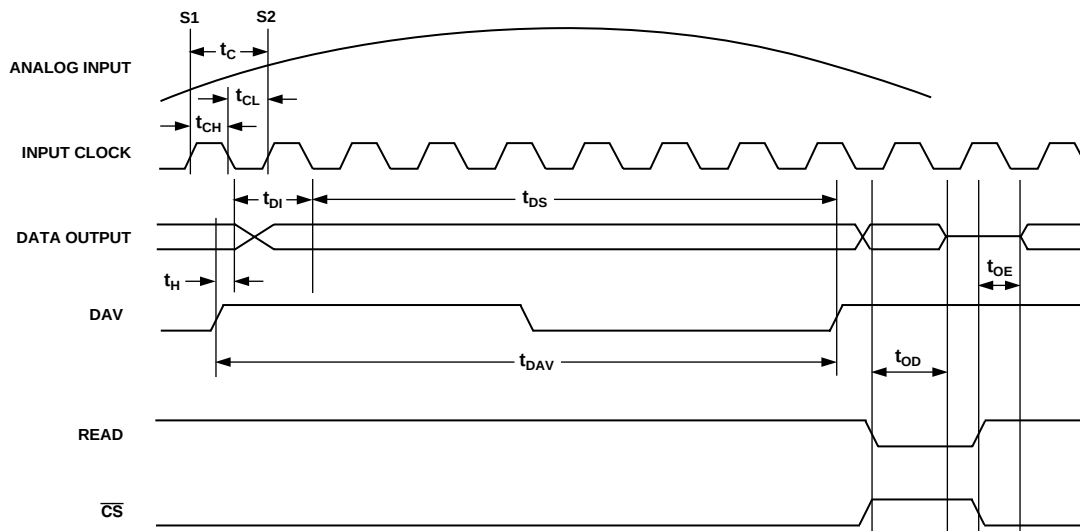
Figure 4. Timing Diagram
