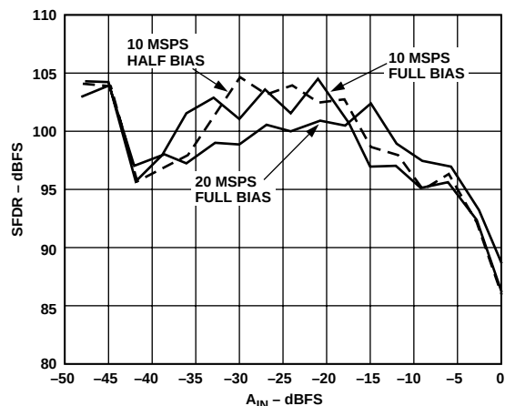
Figure 49. Single-Tone SFDR vs. Amplitude ( f_{IN} = 500 kHz, 2x Mode)
