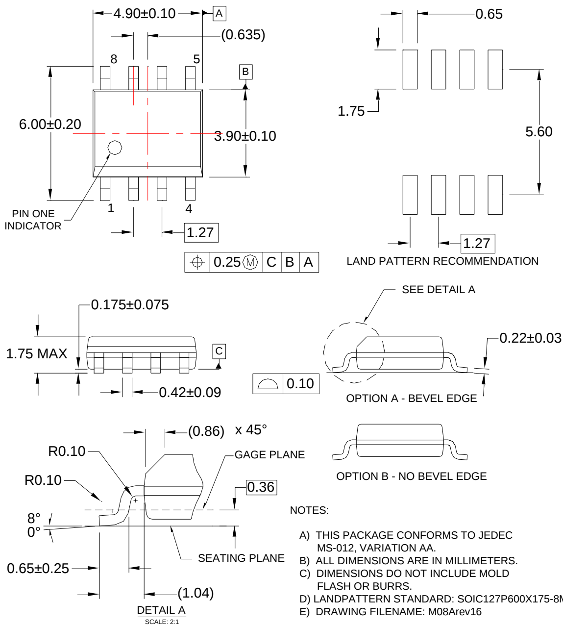
Figure 36. 8-Lead Small Outline Integrated Circuit (SOIC)
