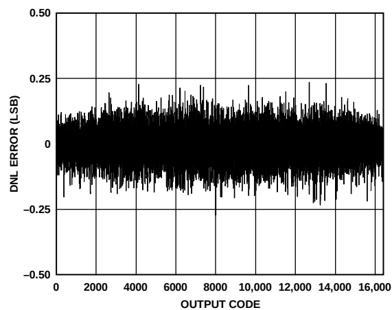
Figure 51. AD9255-125 DNL with f_{IN} = 12.5 MHz
