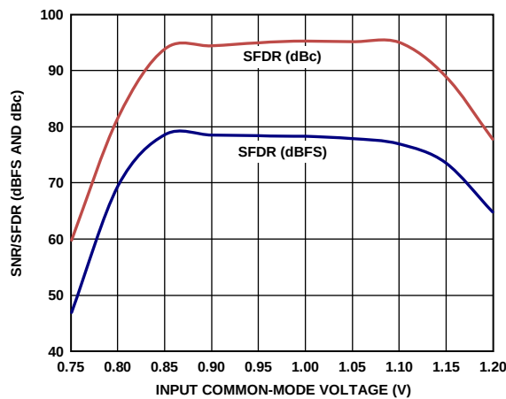
Figure 52. AD9255-125 SNR/SFDR vs. Input Common Mode (VCM) with f_{IN} = 30 MHz
