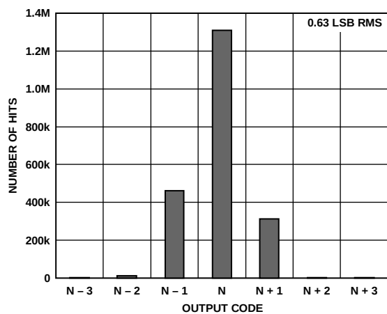
Figure 49. AD9255-125 Grounded Input Histogram
