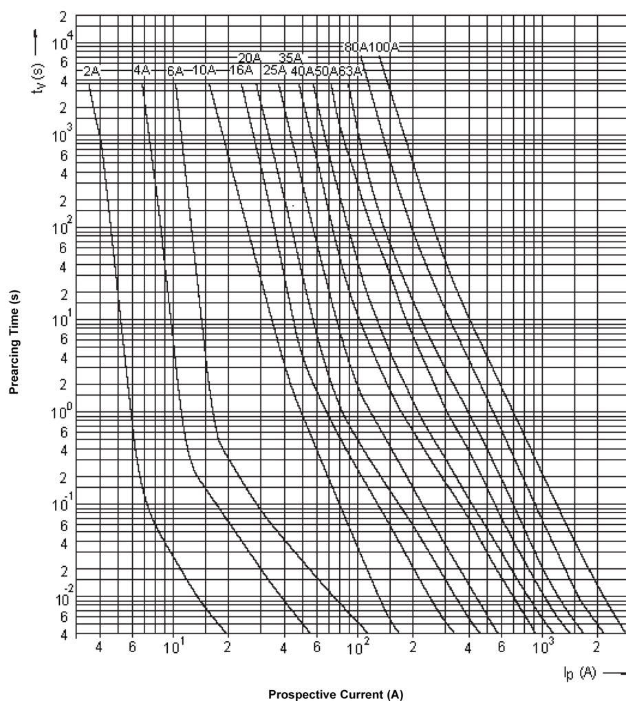
Time Current Characteristics I/t gG
