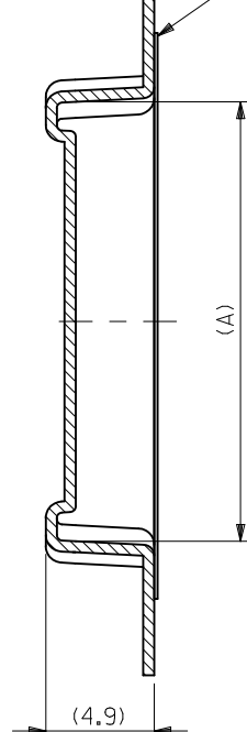
SECT X-X
