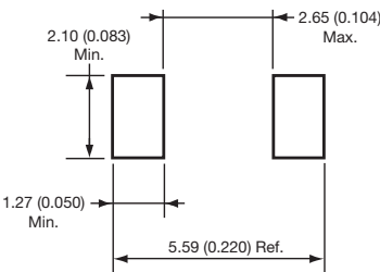
DO-214AA (SMB)
