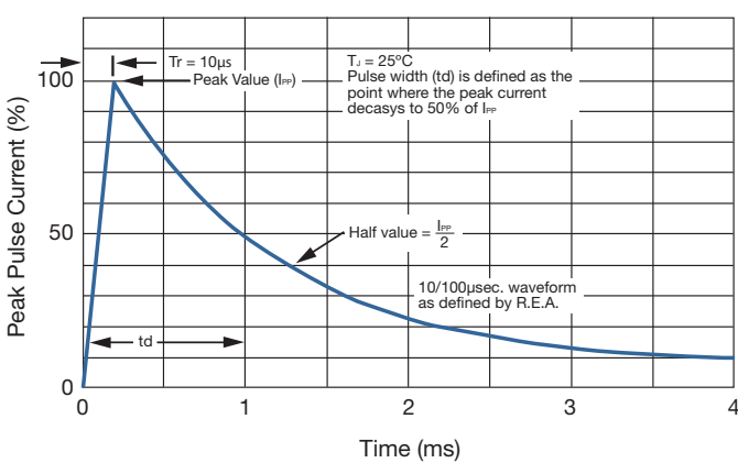
FIG 5. PULSE WAVEFORM
