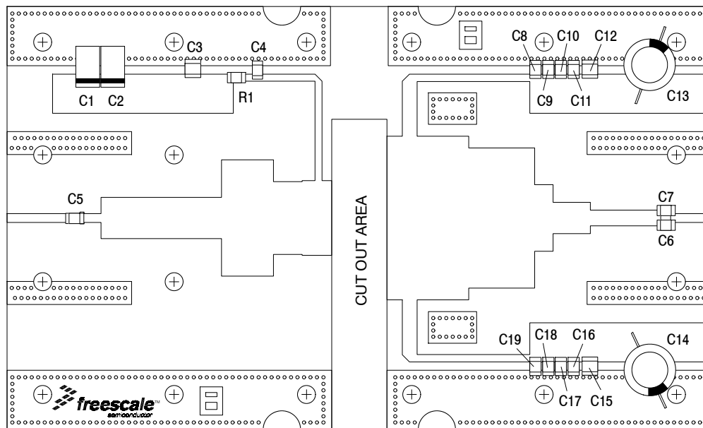
Figure 13. MMRF1005HR5(HSR5) Application Circuit Component Layout — 1300 MHz, CW
