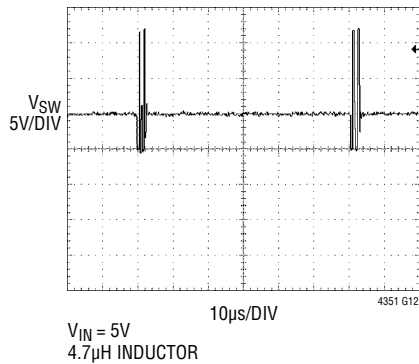
Typical SW Pin Waveform
