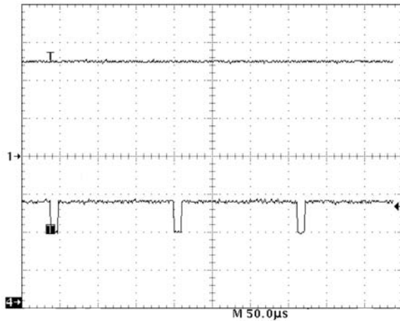
Figure 25. Power Good is Insensitive to Out of Regulation Conditions that are Present for a Duration Less Than the Built In Delay
