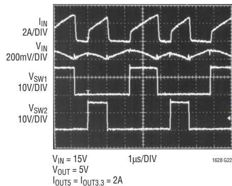
Input Source/Capacitor Instantaneous Current (Figure 14)
