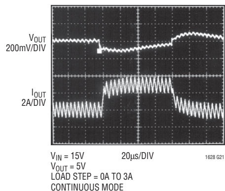
Load Step (Figure 14)
