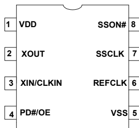
Figure 1. CY25100 8-pin SOIC/TSSOP
