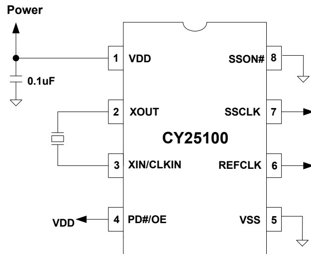
Figure 2. Application Circuit Diagram [4, 5, 6]
