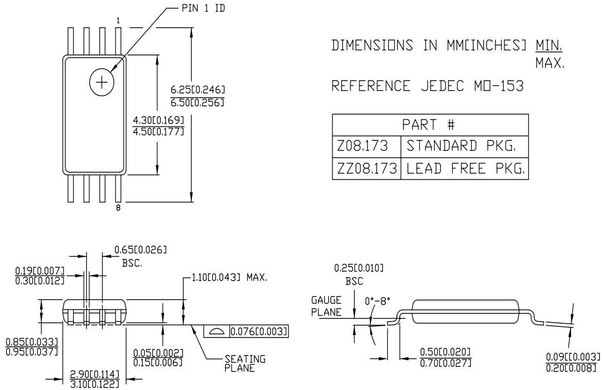
Figure 7. 8-pin TSSOP (4.40 mm Body) Z08.173/ZZ08.173 Package Outline, 51-85093
