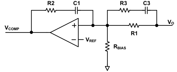
FIGURE 30. TYPE III COMPENSATOR
