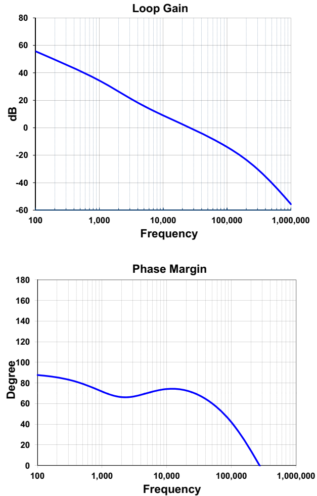
FIGURE 31. SIMULATED LOOP BODE PLOT
