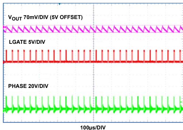
FIGURE 17. V_{IN} 24V, 80mA LOAD, PFM MODE
