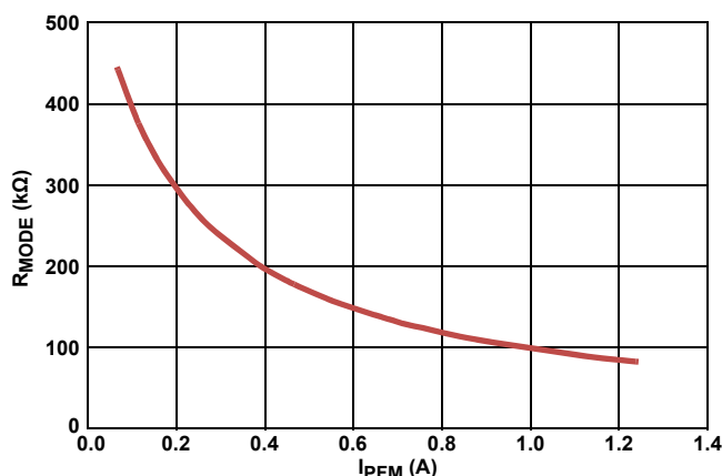
FIGURE 25. R MODE vs I PFM
