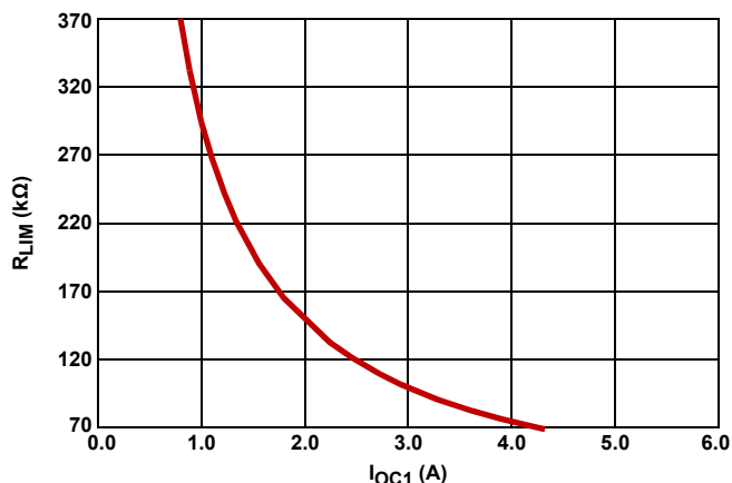
FIGURE 28. R_{LIM} vs I_{OC1}
