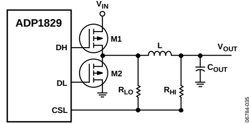
Figure 25. Short Circuit Current Foldback Scheme
