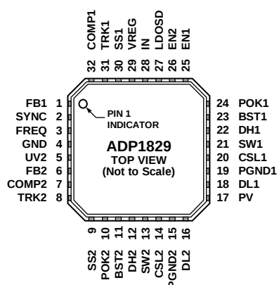
Figure 3. ADP1829 Pin Configuration
