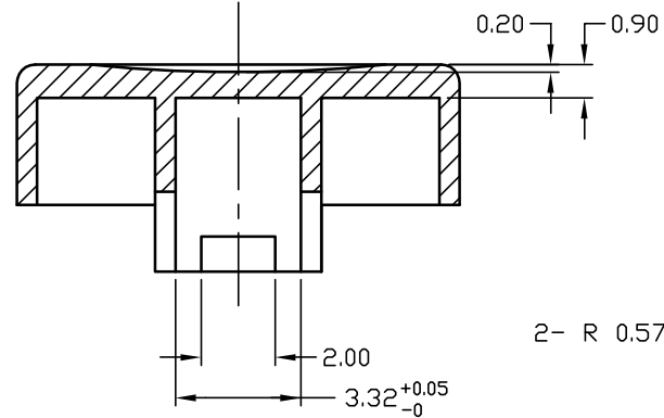
SECTION A-A DETAIL
