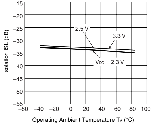
RFC-RF1/RF2/RF3/RF4 ISOLATION vs. OPERATING AMBIENT TEMPERATURE f = 3.8 \text{ GHz}
