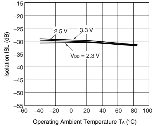
RFC-RF1/RF2/RF3/RF4 ISOLATION vs. OPERATING AMBIENT TEMPERATURE f = 6 \text{ GHz}
