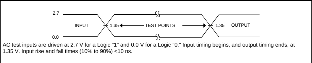
Figure 12. Transient Input/Output Reference Waveform for V_{CC} = 2.7\text{ V}–3.6\text{ V}
