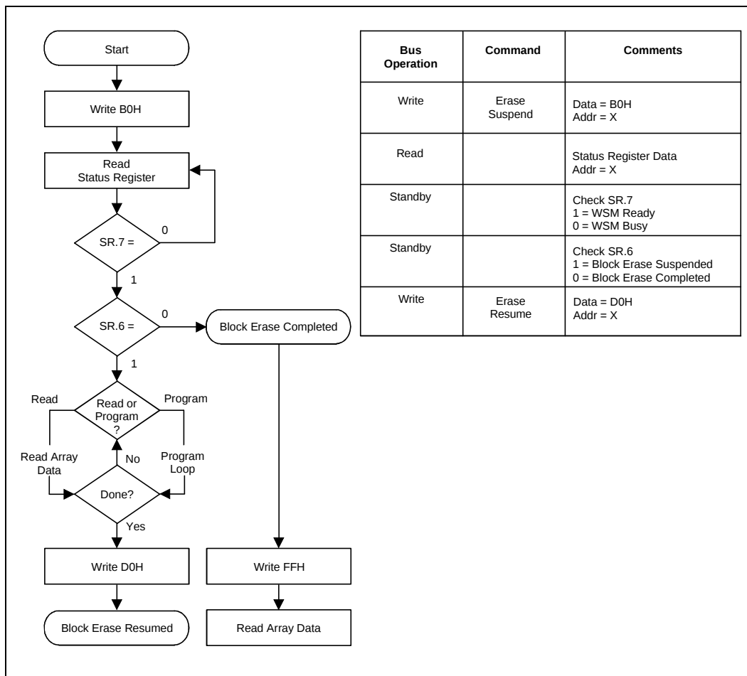
Figure 9. Block Erase Suspend/Resume Flowchart
