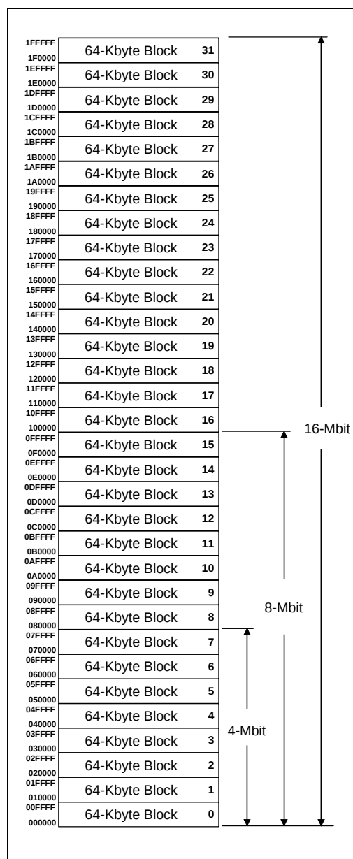
Figure 5. Memory Map
