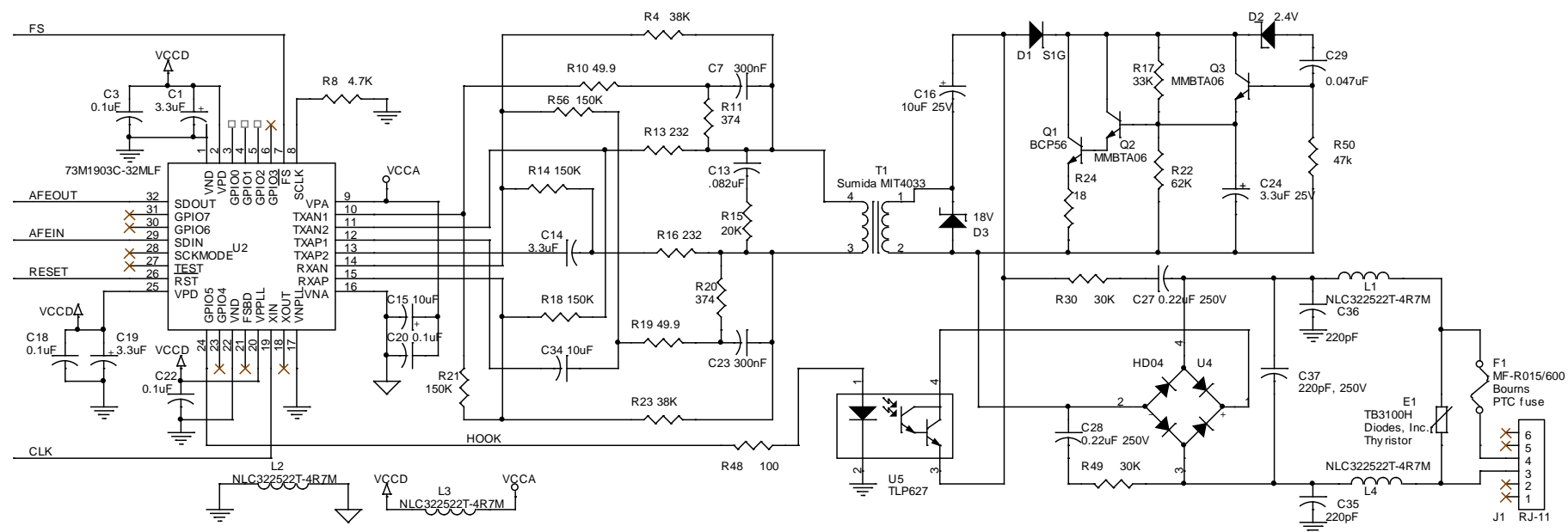
Figure 15: 73M1903C Schematic
