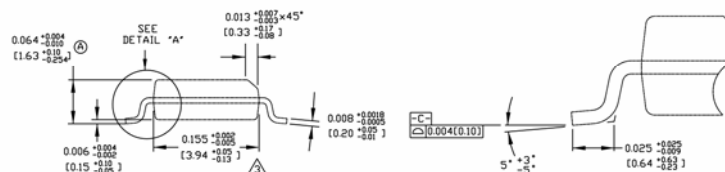
END VIEW
