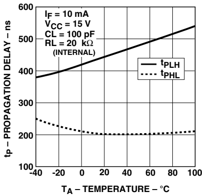
Figure 9. Propagation delay with internal 20\text{ k}\Omega R_L vs. temperature.
