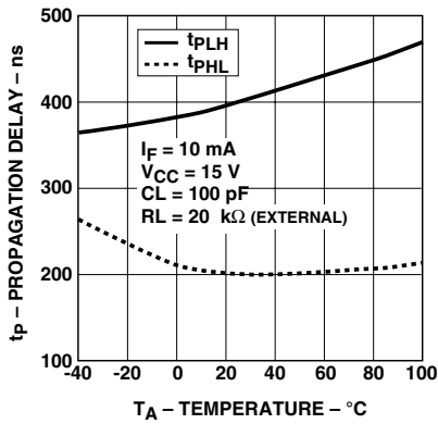
Figure 8. Propagation delay with external 20\text{ k}\Omega R_L vs. temperature.
