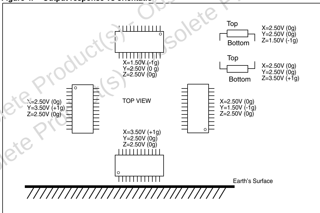
Figure 4. Output response vs orientation
