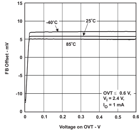
Figure 6. FB Offset vs Voltage ON V_{OUT}
