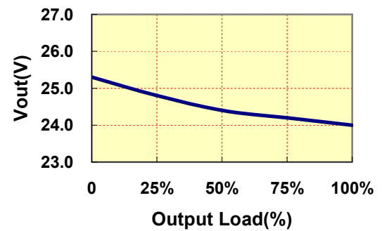
VOUT VS LOAD(24Vout Models)
